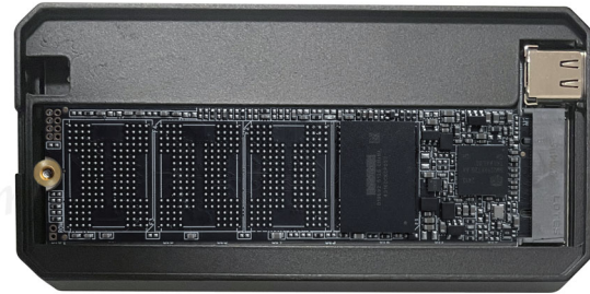
Installed PSSD bottom shell
