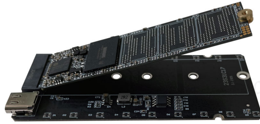
Tilt insertion SSD
